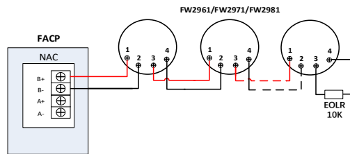
(b) Conventional – Class B with MA panel
