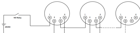
(c) Conventional – Class B with external power supply under Independent Mode
