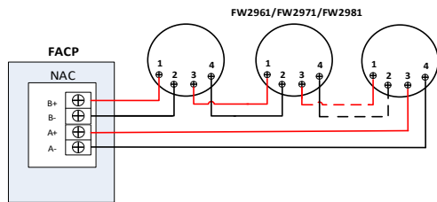
(a) Conventional – Class A with MA panel
