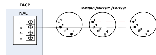
(e) Addressable – Class B with MA panel
